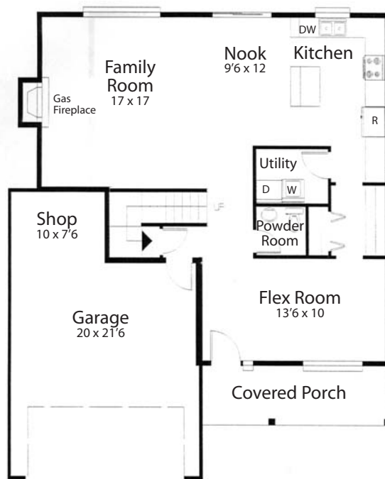
Main Floor Plan 1082 square feet
